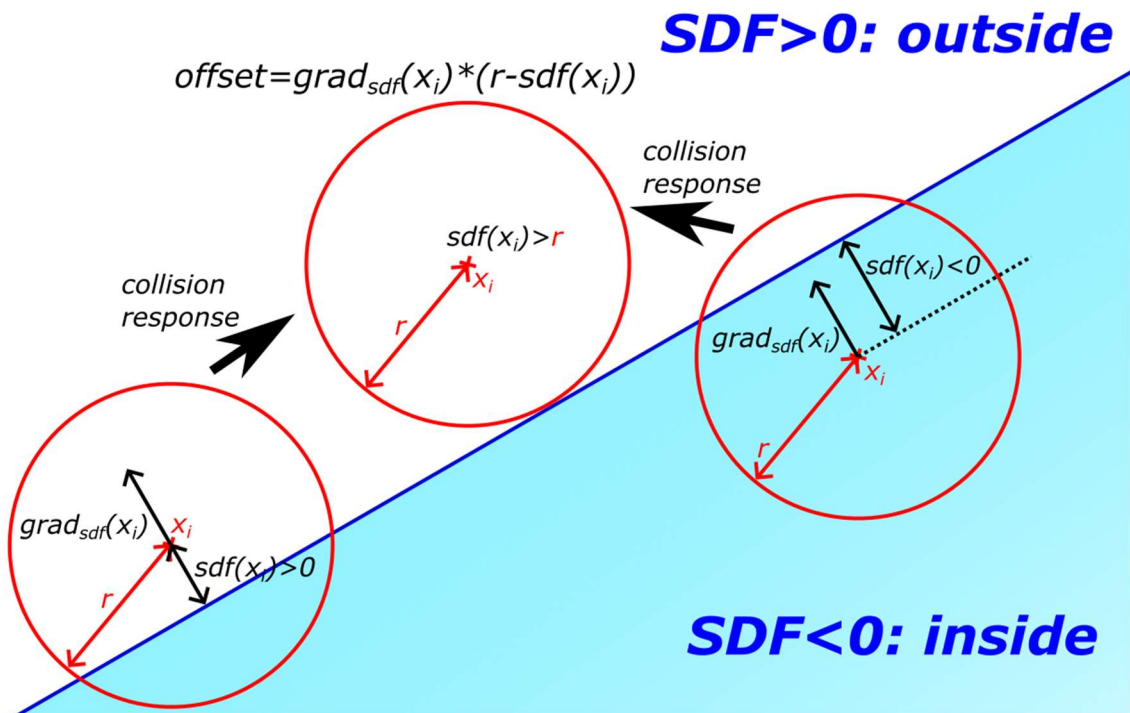
Figure 14: SDF collision detection and response.
